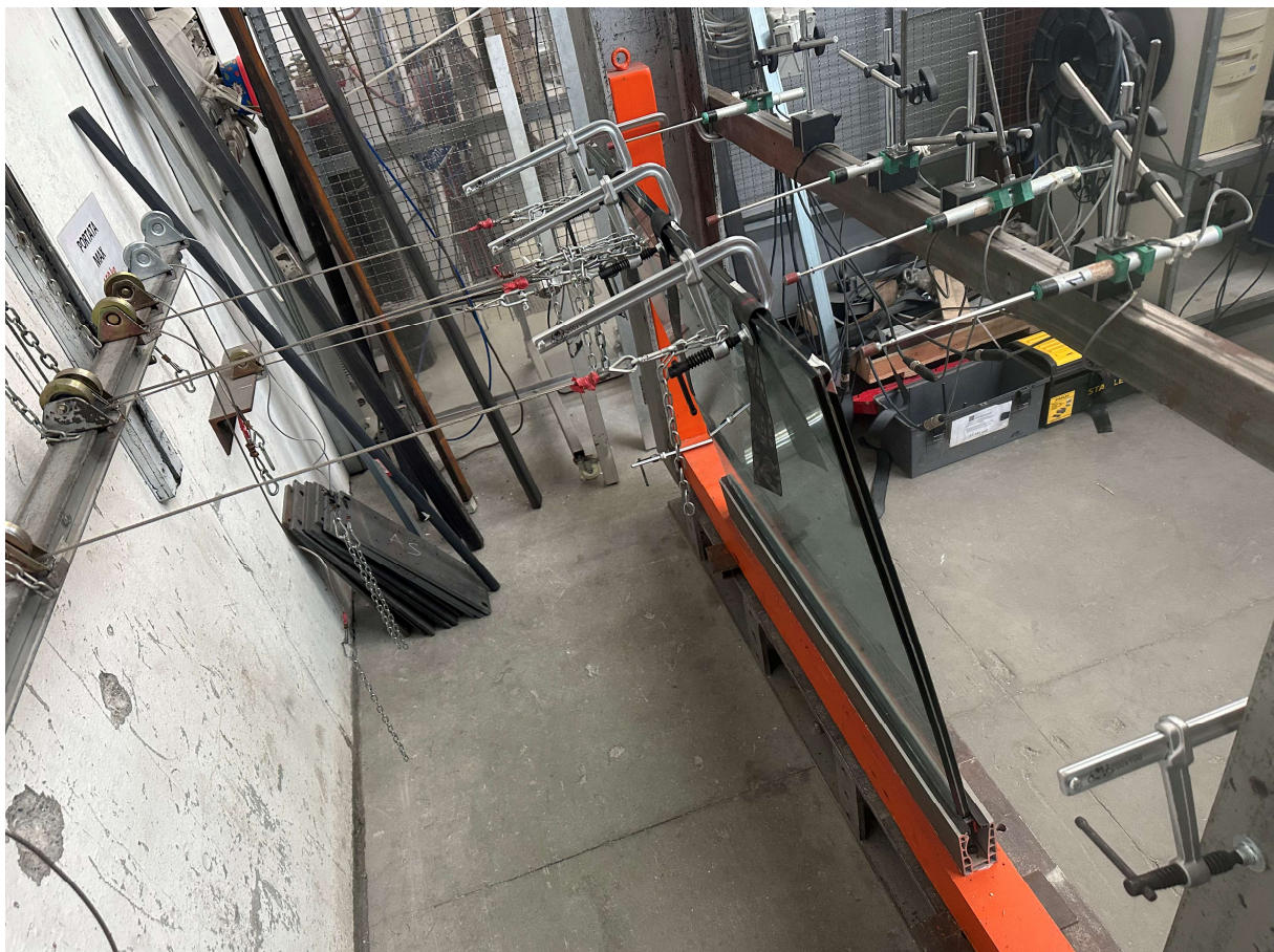
Photograph of the item during resistance to outward horizontal static loading test
